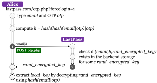
Figure 5: LastPass OTP Creation. Note the absence of any CSRF token in the request in Step 1.
