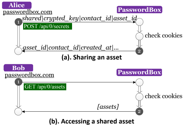
Figure 8: PasswordBox: Sharing an asset. The underlined passwordbox.com on the left indicates that the code making the request runs in the passwordbox.com origin.
