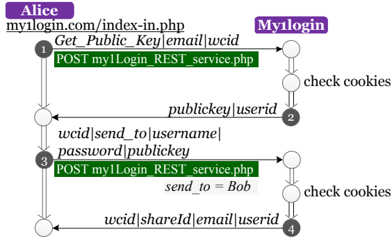
Figure 7: Sharing Credentials on MyIlogin
